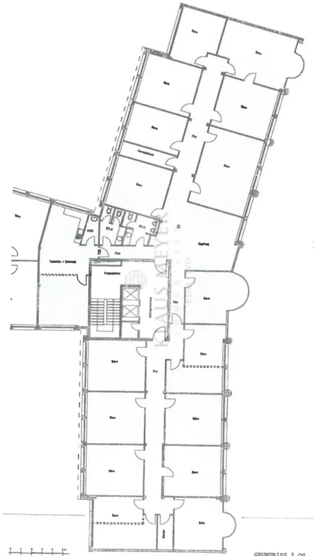
GRUNDRISS 2.0G
