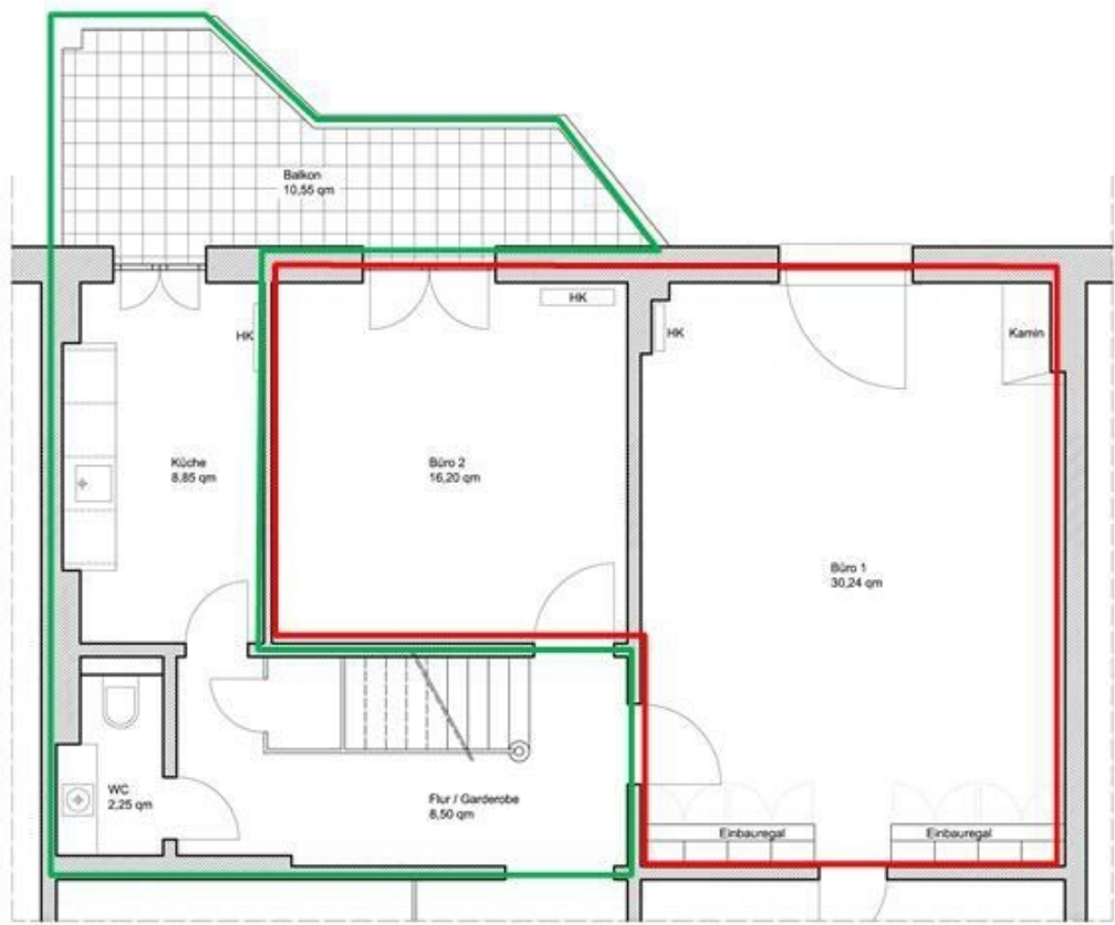
Grundriss 1OG
