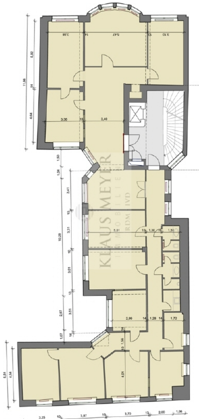
Grundriss 2OG
