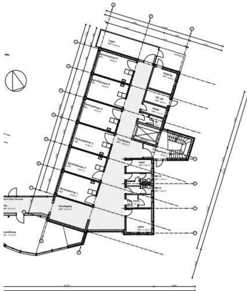
Grundriss EG OF
