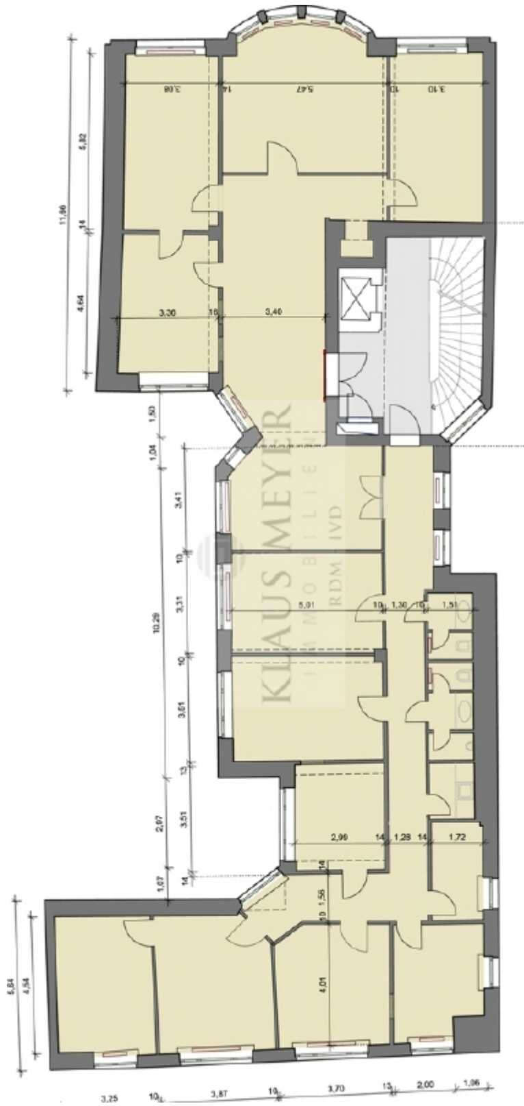
Grundriss 2OG
